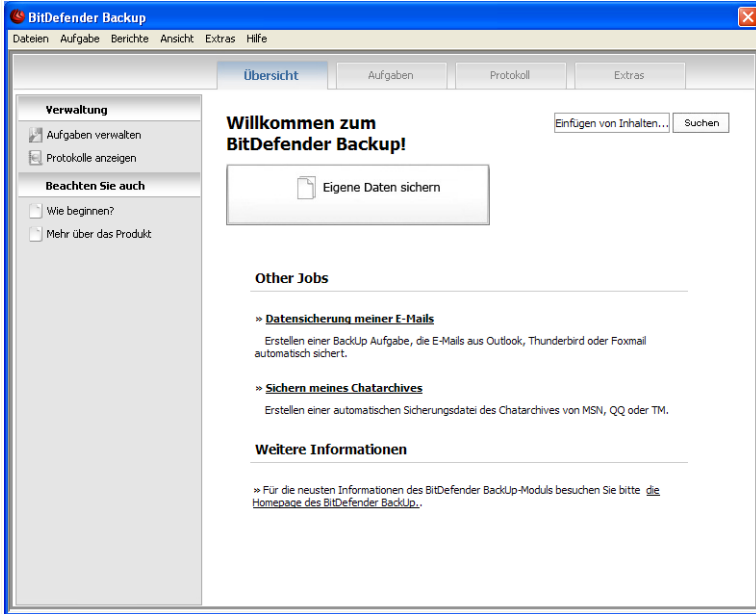
BitDefender Backup
