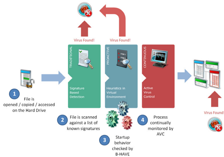
Figure 1: The BitDefender Scanning Sequence
