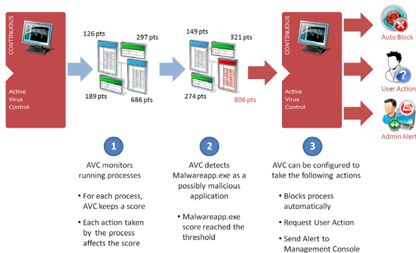
Figure 2: AVC Process Monitoring and Threat Response
