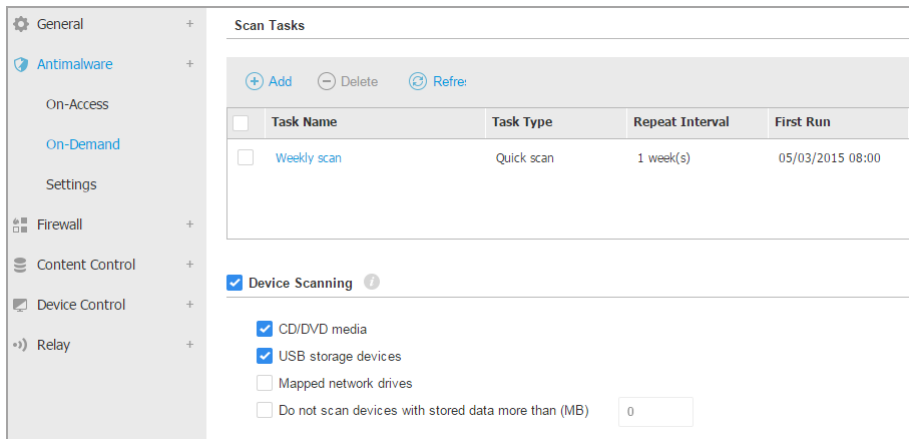
Policies - On Demand Scan Tasks
